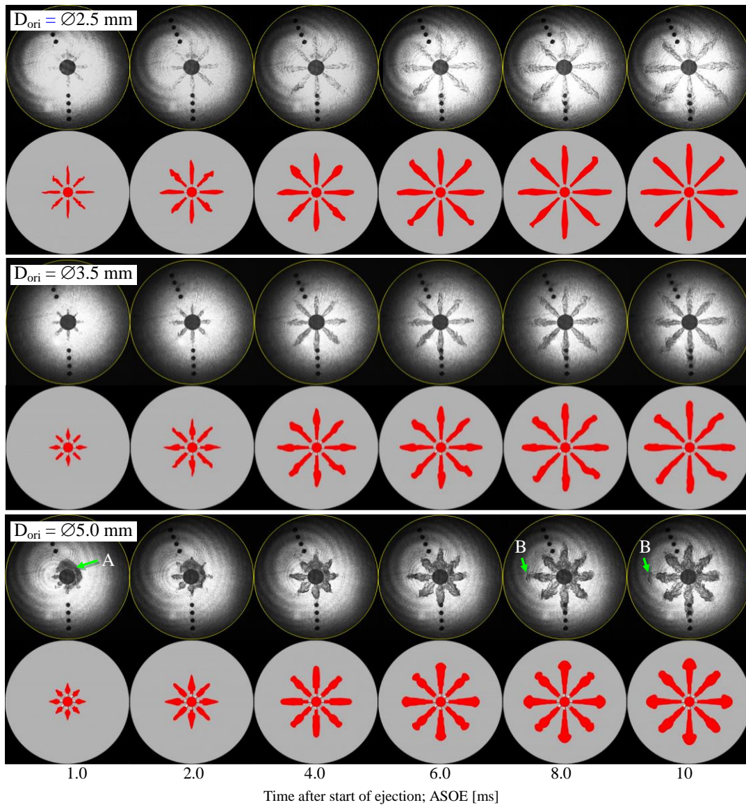
Fig. 10. Effects of orifice diameter; D_{ori} on ejection behaviour of torch flame by PC Tip #4 ( \text{Ø}2.5 mm), #1 ( \text{Ø}3.5 mm), and #5 ( \text{Ø}5.0 mm), respectively with N_{ori} = 8 and V_{PC} in common, in the shadowgraph images (upper row of island) and simulation results (lower row)
