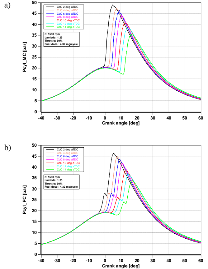
Fig. 7. Example of cylinder pressure waveform with \lambda = 1.25 and different CoC = 2–14°CA aTDC: a) in main chamber; b) in pre-chamber
