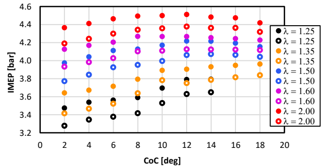
Fig. 13. The value of the indicative mean effective pressure as a function of the center of combustion for the main and pre-chamber ( \bullet – MC, \bullet – PC)
