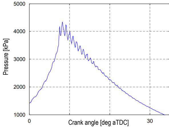
Fig. 1. Cylinder pressure with knocking combustion ( \varepsilon = 12:1 ; n = 900 rpm; \lambda = 1 ) [31]
