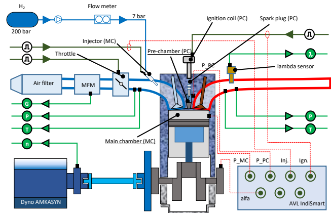
Fig. 5. Layout of engine and test apparatus
