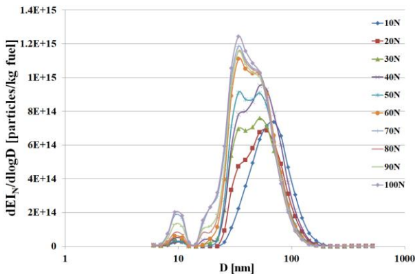
Fig. 9. Number-based particle size distribution
