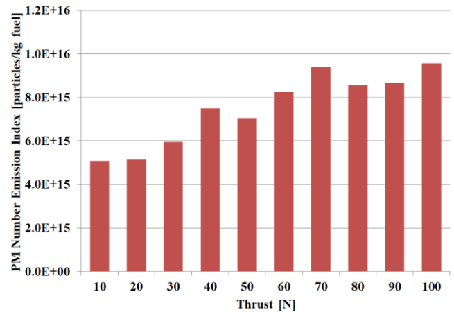
Fig. 7. PM number emission index
