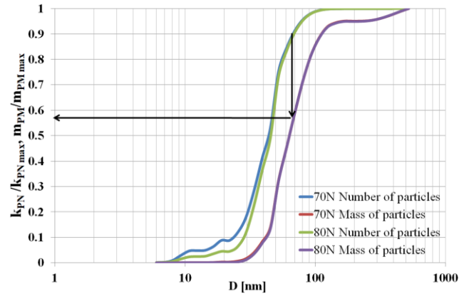
Fig. 15. Cumulative values of the relative particles number and relative mass of particulate matter for 70 N and 80 N
