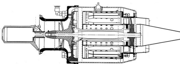
Fig. 1. Illustrative diagram of GTM-120 [1]
