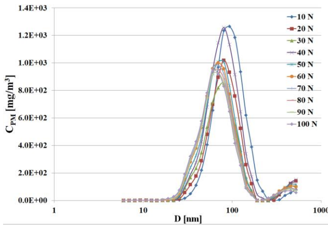
Fig. 4. Particles mass concentration for measurement points
