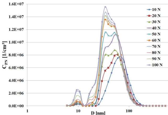
Fig. 3. Particles number concentration for measurement points
