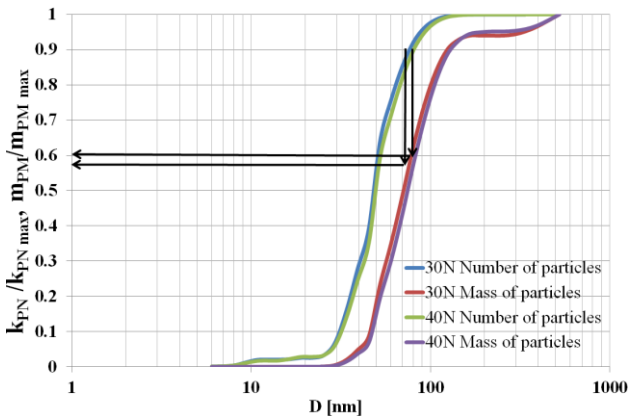
Fig. 13. Cumulative values of the relative particles number and relative mass of particulate matter for 30 N and 40 N
