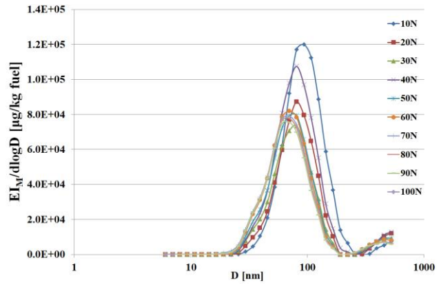
Fig. 10. Mass-based particle size distribution
