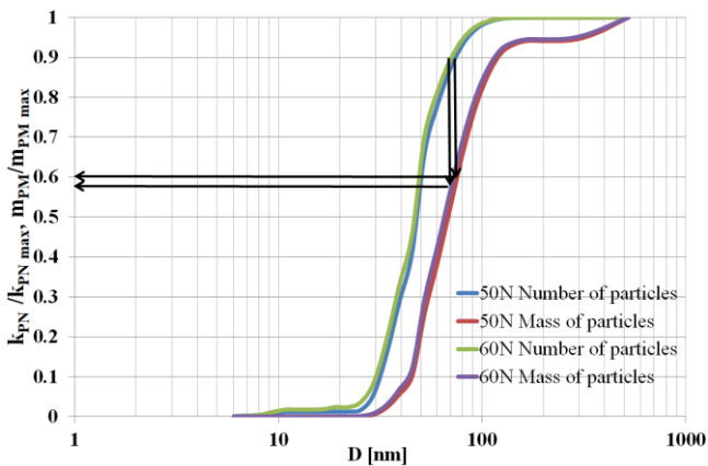
Fig. 14. Cumulative values of the relative particles number and relative mass of particulate matter for 50 N and 60 N
