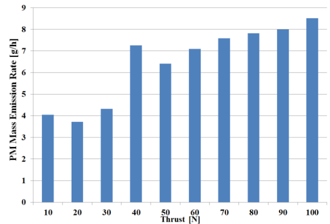
Fig. 6. PM mass emission rate
