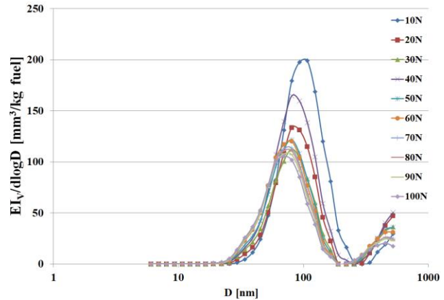
Fig. 11. Volume-based particle size distribution
