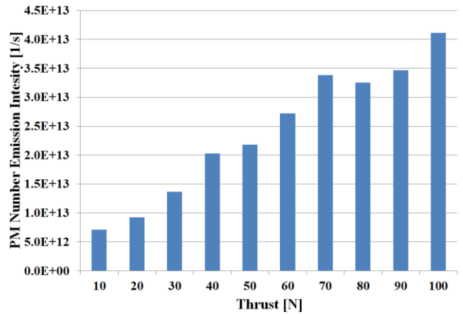
Fig. 5. Intensity of particles number emission
