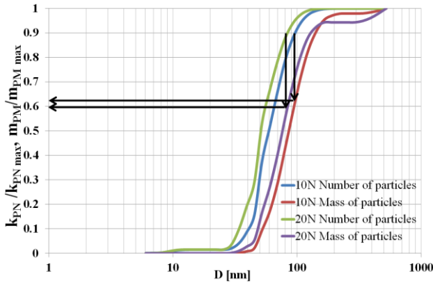
Fig. 12. Cumulative values of the relative particles number and relative mass of particulate matter for 10 N and 20 N
