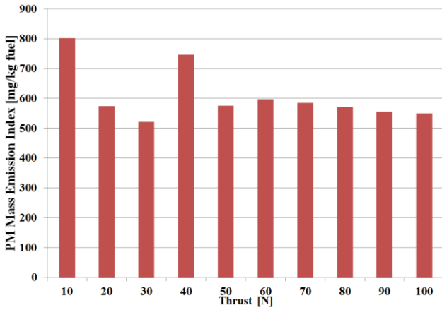
Fig. 8. PM mass emission index
