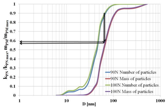
Fig. 16. Cumulative values of the relative particles number and relative mass of particulate matter for 90 N and 100 N
