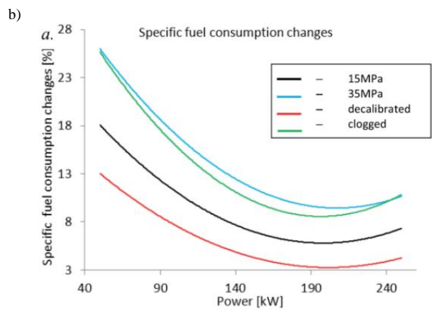
Fig. 8. Changes of combustion pressure of gas mixture in engine cylinder (a) and specific fuel consumption (b) for the experimental study consists of 5 stages, at different simulated malfunctions of the fuel injector installed in 2nd cylinder of the ship engine, where properly opening pressure is 25 MPa [27]
